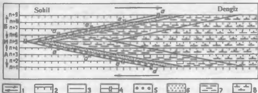
72-rasm. Uchinchi fatsial zonallik qonunini tushuntiruvchi chizma.
