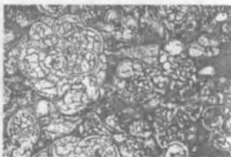
56-rasm. Foraminijerali ohaktoshning mikrofotosurati
