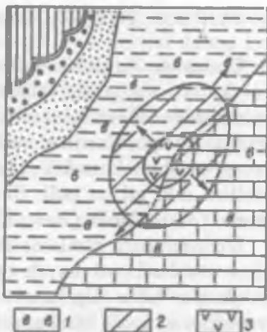
75-rasm. Beshinchi fatsial zonallik qonunini tushuntiruvchi chizma.
