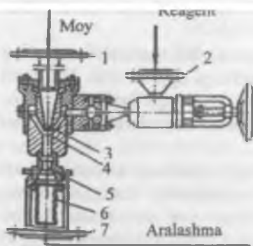
1.2-rasm. Reaktor-turbulizator.
