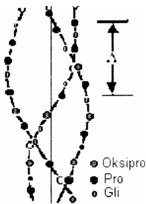
5-rasm. Kollagen oqsili molekulasining tuzilishi.
