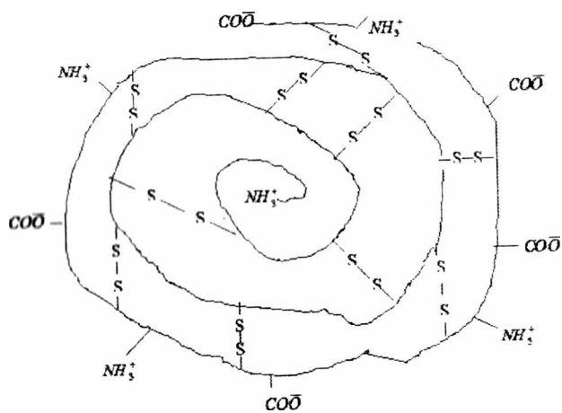
4-rasm. Oqsillar molekularining uchlamchi tuzilishi
