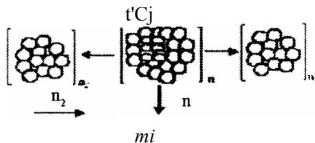
11-rasm. Sovuq suv molekulari agregatining harorat ta'sirida kichik agregatlarga parchalanishi.
