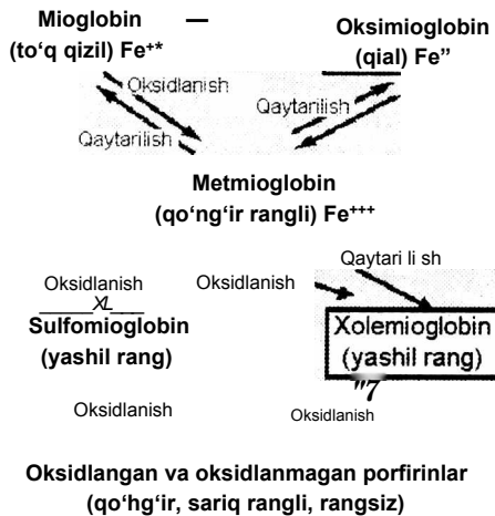
45-rasm. Go'sht mioglobinining mikroblar ta'sirida oksidlanishi
