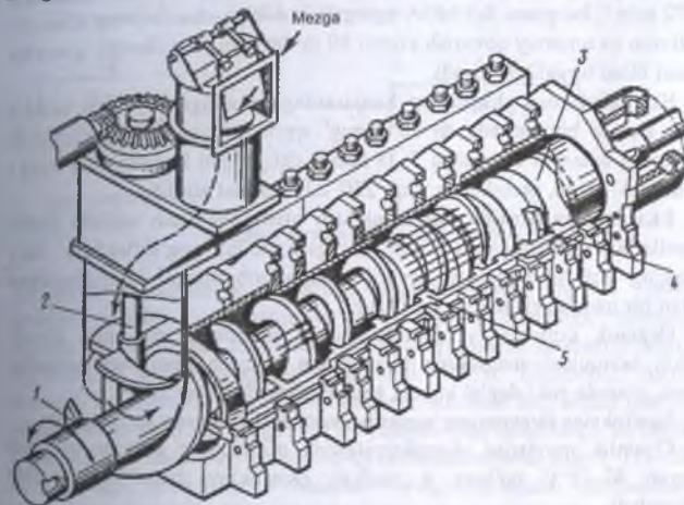
5.8-rasm. Shnekli press.
