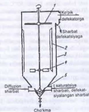
6.6-rasm. Optimal olddefekatsiyalash apparati.
