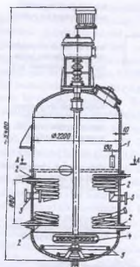
5.25-rasm. Turbina-aralashtirgichli reaktor.
