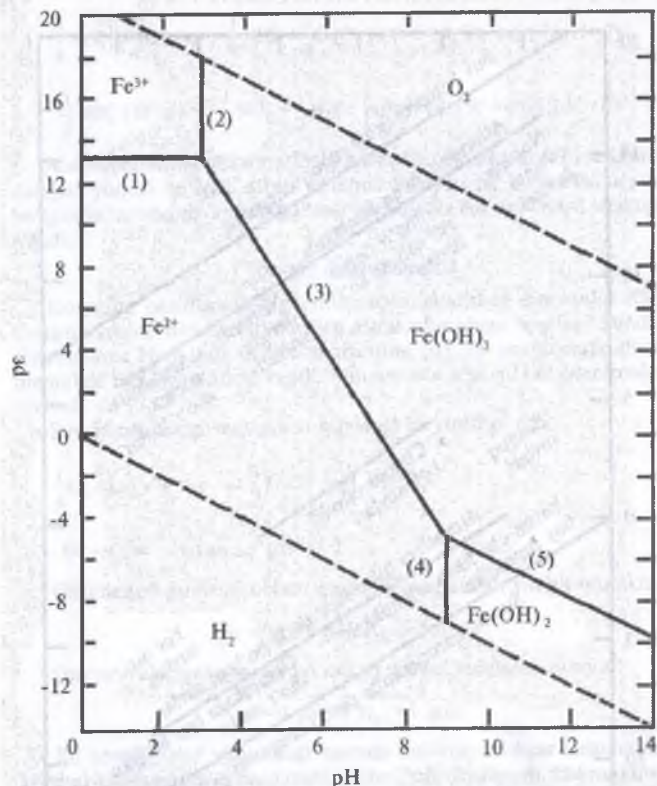
25-rasm. \text{Fe}^{2+} - \text{Fe}^{3+} sistemasi uchun p\epsilon/\text{pH} diagrammasi, temirning miqdori 1,0 \cdot 10^{-5} \text{ M} .
