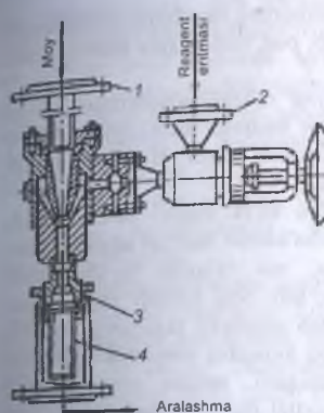
5.18-rasm. Reaktor-turbulizator.
