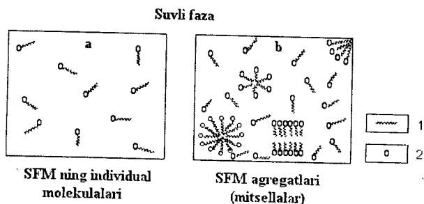
23-rasm. Suvda sirt-faol moddalar (SFM) molekularining sxematik ko'rinishi.
