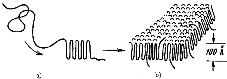
101 – rasm. Polimer kristall lamellari hosil bo'lish jarayonida zanjir taxlanishini tasvirllovchi sxema. a – polimer monokristalli hosil bo'lish jarayonida makromolekula zanjirining taxlanishi; b – polimer kristallik lameli tekisligiga perpendikulyar joylashgan taxlangan makromolekula zanjiri.
