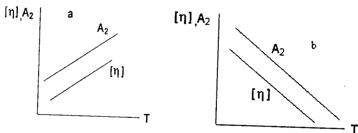
67-rasm. YuKEH (a) va QKEH (b) sistemalar uchun [\eta] va A_2 larning haroratga bog'liqligi.
