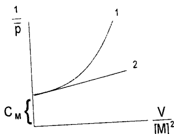
5-rasm. \frac{1}{P} - \frac{V}{[M]^2} bog'liklik grafiqi;
