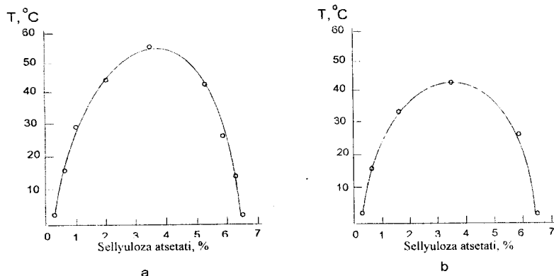
43-rasm. Holat diagrammalari: a – sellyuloza atsetati – xloroform; b – sellyuloza atsetati – dixlorektan
