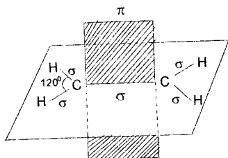
36-rasm. Etilen molekulasini modeli
