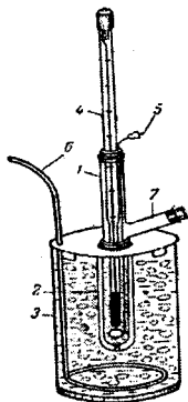
69-rasm. Polimerlar molekulyar massasini krioskopik usulda topish uchun asbob: 1-yon shohobchali krioskopik yacheyka; 2-probirka; 3-stakan; 4,6-aralashtirgichlar; 5-Bekman termometri; 7-yutuvchi.
