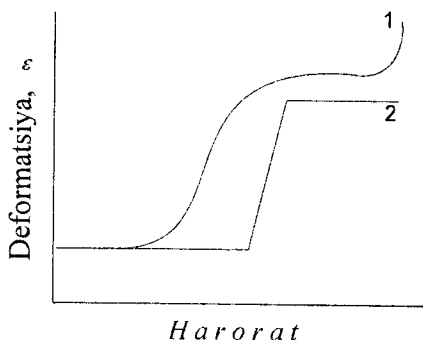
88-rasm. Polimerlarning termomechanik egri chiziqlari; 1 – amorf polimer; 2 – kristall polimer.
