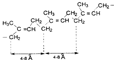
Trans-izomer (guttapercha)
