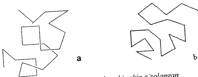
56-rasm. O'z-o'zicha kesishuvchi erkin a'zolangan zanjir (a)
