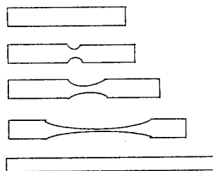
116-rasm. Kristall polimerni cho‘zganda bo‘yinch hosil bo‘lishi.
