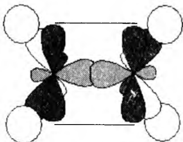
1.7-Rasm. Etilen molekulasida gibridd orbitallarning hosil bo'lishi
