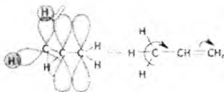
propen
