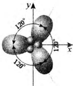
1.7-Rasm. Etilen molekulasida gibridd orbitallarning hosil bo'lishi
