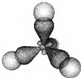
1.4-Rasm. Metanda gibrid orbitallarning yo'nalishlari
