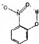
o-nitrofenol
