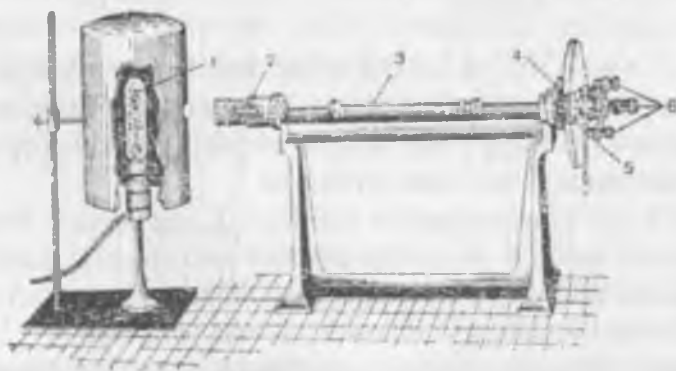
12- rasm. Polarimetr:
