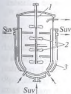
31- rasm. Parrakli aralashtirgichi bo'lgan reaktor.
