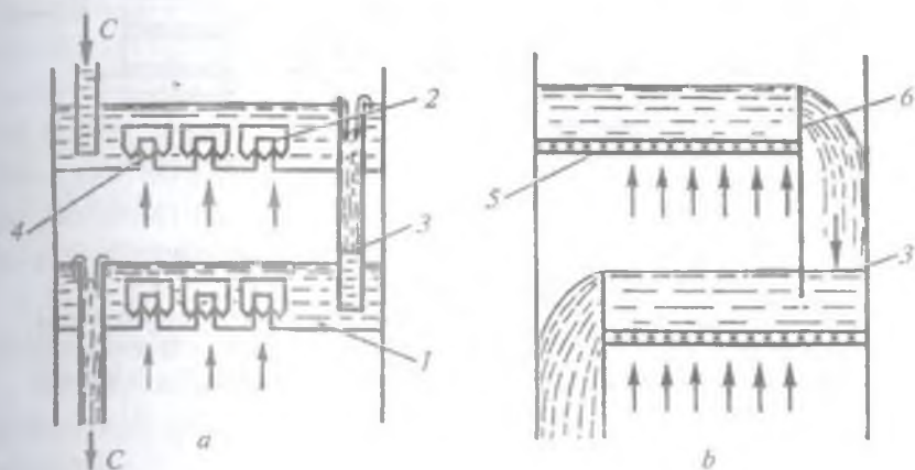
37- rasm. Barbatayli apparat tokchalarining (tarelka) sxemasi.
