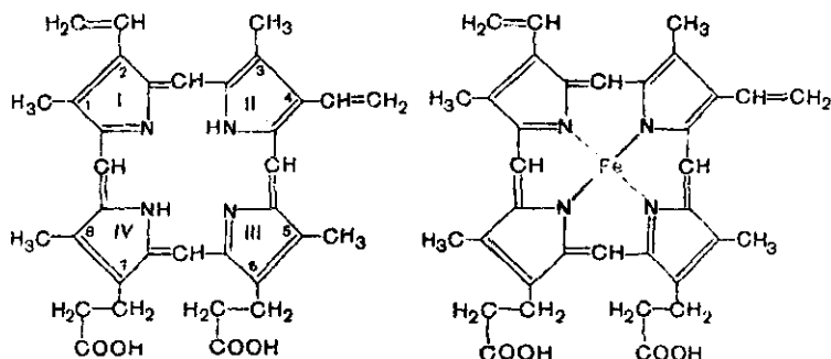
Protoporfirin-IX
