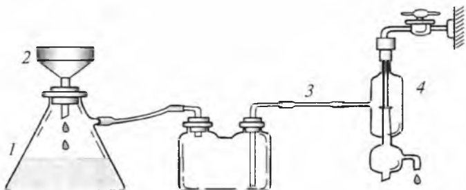
14-rasm. Past bosimda filtrlash.
