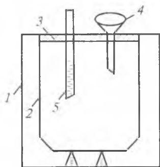
25-rasm. Kalorimetr:
