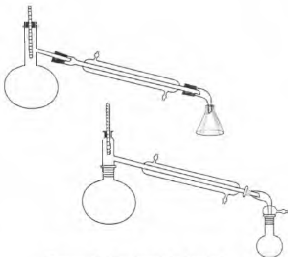
17-rasm. Oddiy sharoitda haydash.
