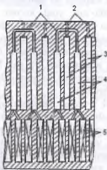
7-rasm. Koks pechining sxemasi: 1-o'tish kanallari; 2-truba; 3-kokoslash kameralari; 4- isitish moslamalari; 5- regeneratrlar.
