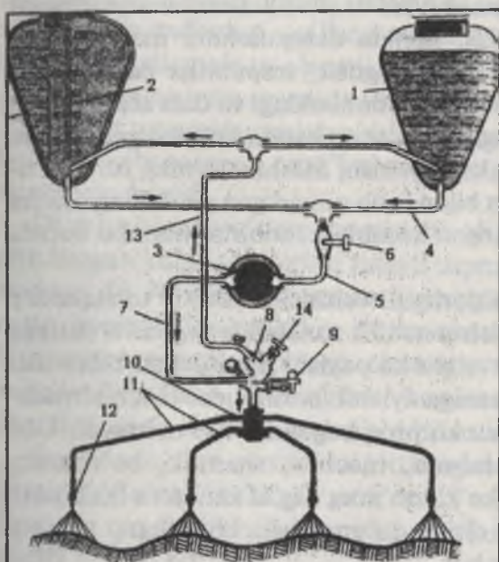
9-rasm. PGS-2.4 moslamasining texnologik sxemasi:
