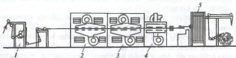
2.17- rasm. Stabillovchi quritish-kengaytirish mashinasining chizmasi:
