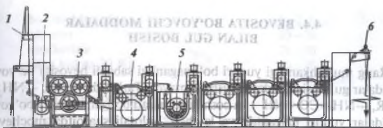
4.12- rasm. «Arioli» universal yuvish mashinasining chizmasi:
