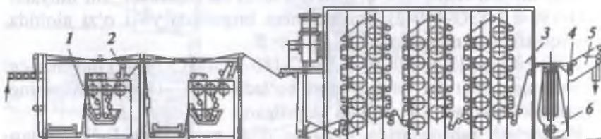
5.9- rasm. LKC-220-21 liniyasining texnologik chizmasi:
