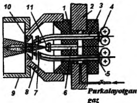
9.12-rasm. Elektroyoyli metallizatorning purkash kallagining sxemasi:
