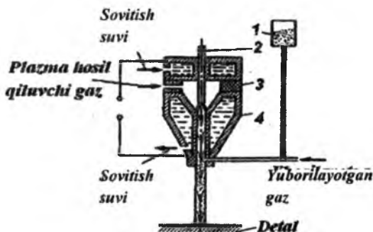
9.14-rasm. Plazmali metallizatsiyalash gorelkasining sxemasi: 1 – kukun dozatori; 2 – katod; 3 – izolyatsion qo'yilma; 4 – anod (soplo).
