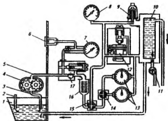
11.9-rasm. KH-4815M stendida nasosni sinash sxemasi:
