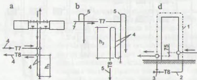
9.6a, b, d-rasm. 1 – havo quvuri; 2 – eshik ostidan o'tkazilgan quvur; 3 – uchtalik tiqindon; 4 – suv zulfini; 5 – kalach; 6 – kondensat tirgak
