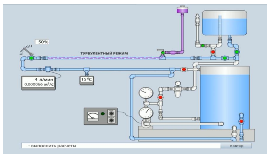
6.1.-rasm. Tajriba qurilmasining tuzilish chizmasi
