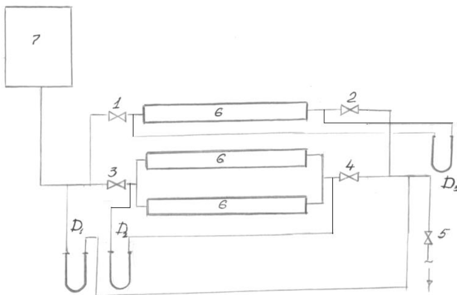
Fig.6.1 Scheme of the laboratory installation.
