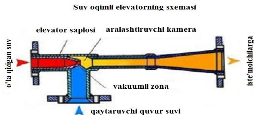
2.1-rasm. Elevatorning tuzulishi.
