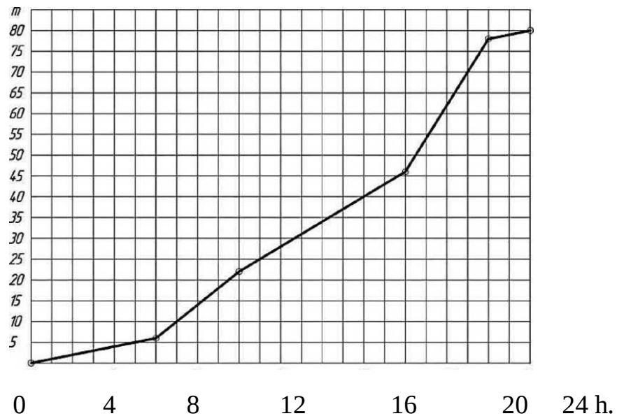
Fig. 1.4 Dynamics of consumption of hot water during the day (example calculation)
