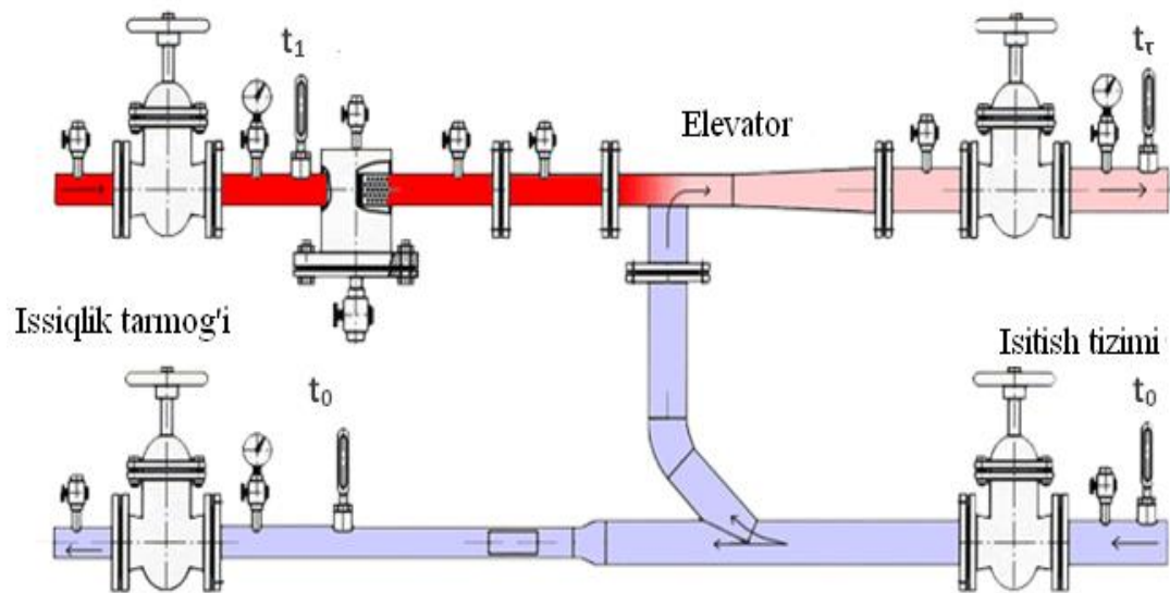
2.3 –rasm. Elevator tugunining sxemasi
