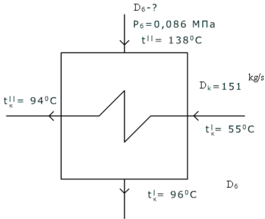
Fig.3.2 Calculation scheme of the low pressure heater.
