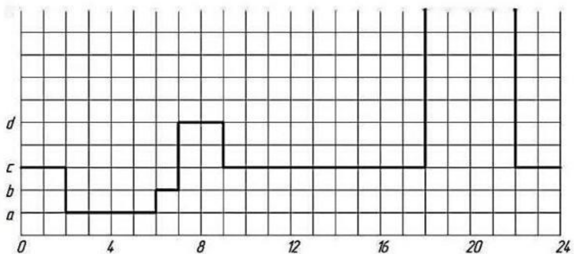
Figure 1.2 Schedule of daily consumption of hot water (task)
