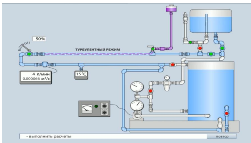
Fig.6.2 Scheme of the laboratory installation.
