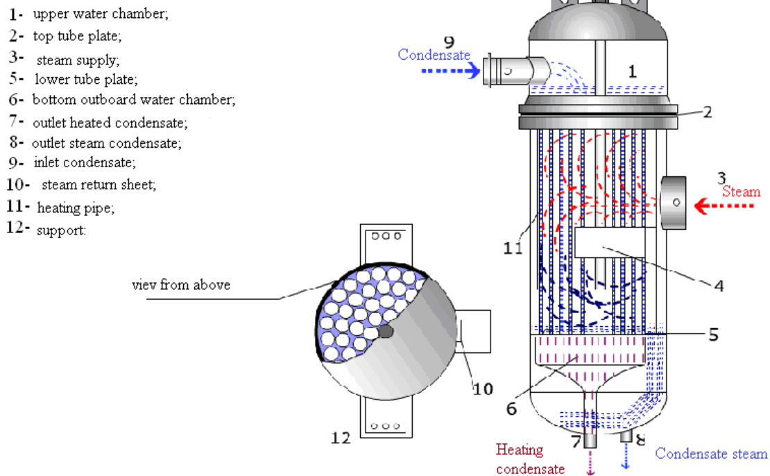
Fig. 3.1 Low-pressure heater circuit.
