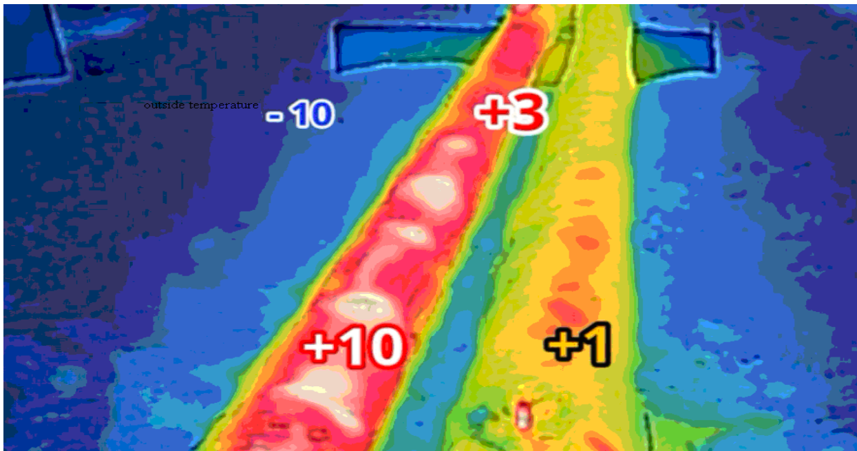
Fig.4.1 Insulated Piping System
