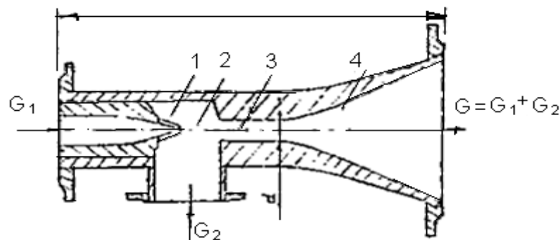
Fig.2.2 Construction of the elevator
