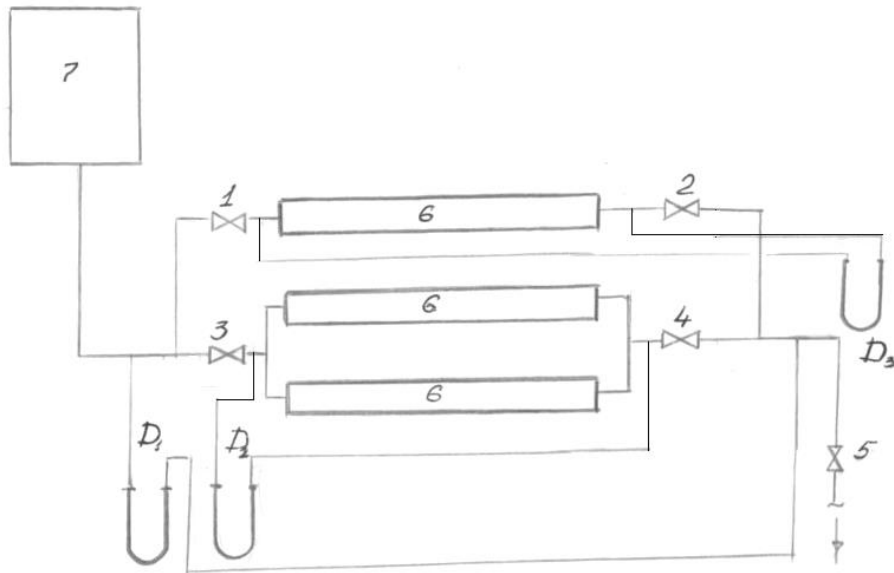
Fig.5.2 Experimental installation scheme
