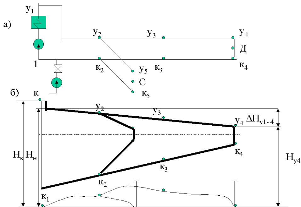
Fig.5.1 The design scheme (a) and piezometric graph (b) of a two-pipe water system of heat pipes.
