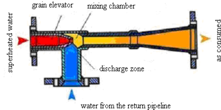
Fig.2.1 Scheme of water-jet elevator.
