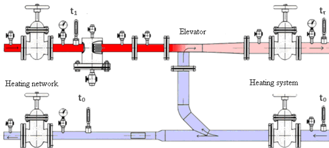
Fig.2.3 Scheme of the elevator assembly.
