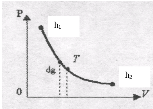
2.3- rasm. P-v diagrammada entalpiyaning o'zgarishi
