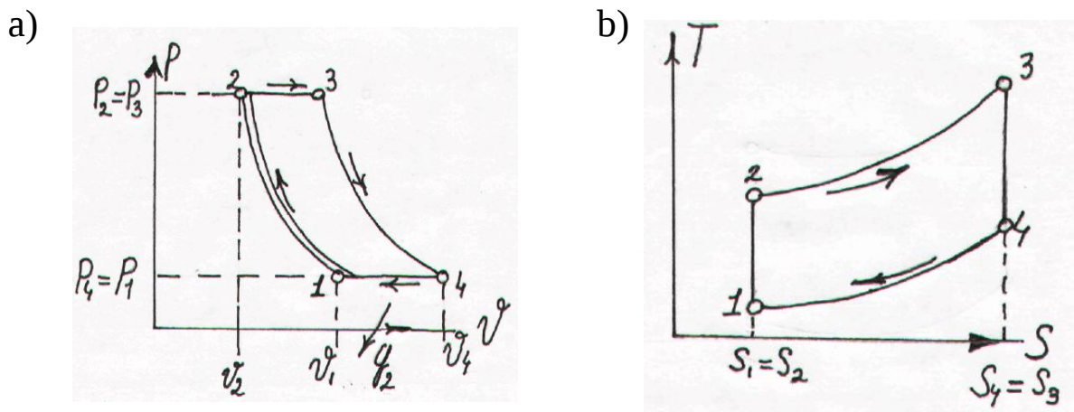
13.1-rasm. a) P=\text{const} gaz turbina qurilmasining P-v diagrammasi b) P=\text{const} gaz turbine qurilmasining T-s diagrammasi
