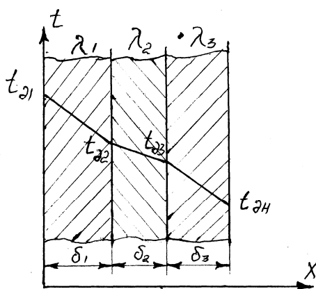
6.3 –rasm. Uch qatlamli devor
