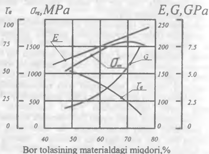
2.3-rasm. Materialdagi bor tolasing miqdorining material mustahkamligiga ta'siri: E – bikirlik moduli; \sigma_{\sigma} – egilishdagi mustahkamlik; G – kesilishdagi moduli; \tau_{\tau} – kesilishdagi mustahkamligi
