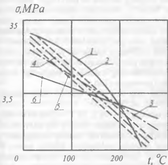
3.3-rasm. Qizdirish haroratining rezina mustahkamligiga ta'siri: 1 – NK; 2 – xloropen; 3 – butilkauchuk; 4 – SKS; 5 – SKN; 6 – SKT.
