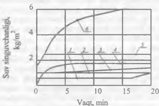
1.5-rasm. Qutubsiz termoplastik plastmassalarning suv singuvchanligini ko'rsatuvchi diagramma: 1 – SEP; 2 – PEND; 3 – PEVD; 4 – ftoroplasti – 4; 5 – polistirol; 6 – selyuloza treatsetat
