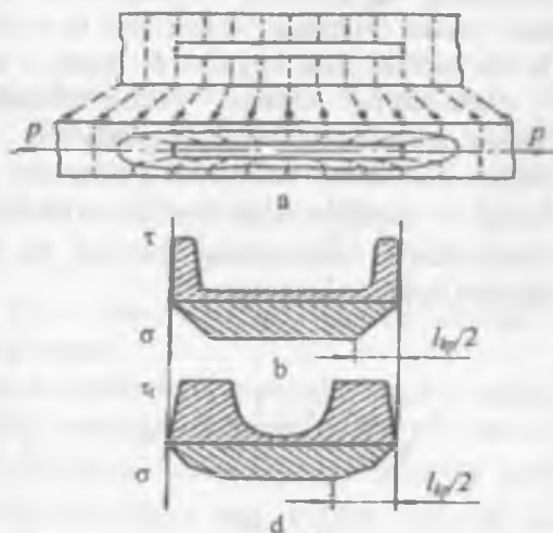
6.1-rasm. Matritsa va tolalarning birgalikdagi (a) deformatsiyalanish sxemasi hamda (b) \tau – urunma, \sigma – normal kuchlanishlarning (d) plastik bikrlik hududidagi epyurasi
