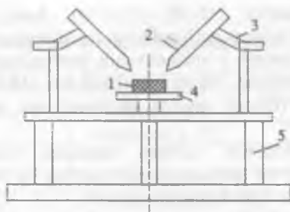
8-rasm. Plastmassalarni uchqunbardoshligini sinash uskunasining sxemasi:
