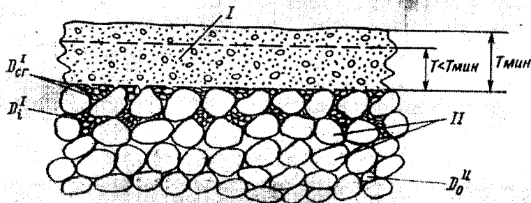
3.8-rasm. Filtr qatlamini tutashishi.
