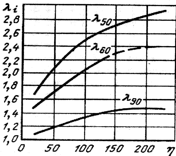
3.5-rasm. qum-shag'al gruntlar uchun \alpha = f(\lambda_i) grafigi
