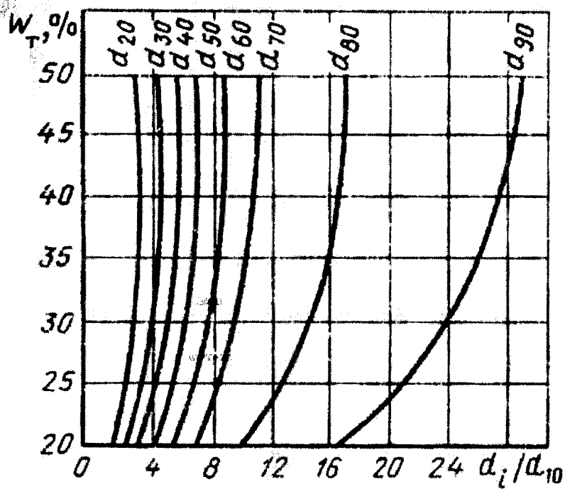
3.6-rasm. d_i / d_{10} = f(W_T) grafigi
