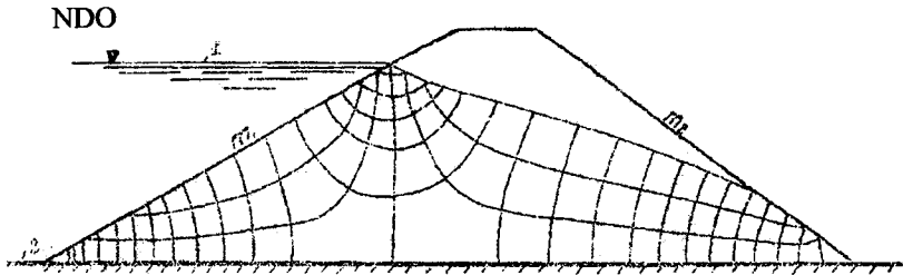
1.1-rasm. Suv omborida suv sathi birdaniga pastlaganda filtratsiya oqimini harakat sxemasi
