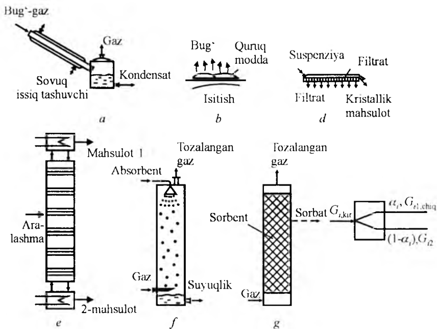
5.12-rasm. Oqimlarning ajratilish sxemalari: a – kondensatorlarda; b – quritgichda; d – filtrda; e – rektifikatsion kolonnada; f – absorberda; g – adsorberda, h – KTS hisobiy elementi bo‘lmish murakkab ajratgich.
