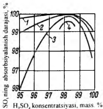
4.20-rasm. Turli temperaturalarda monogidrat absorberida \text{SO}_3 ning absorbsiyalanish darajasi: 1– 60^\circ\text{C} da; 2– 80^\circ\text{C} da; 3– 100^\circ\text{C} da; 4– 120^\circ\text{C} da.
