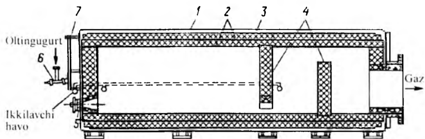
4.9-rasm. Changlangan holatdagi (forsunkali pech) suyuq oltimgugurtni yondirish uchun pech:
