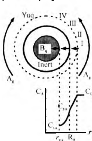
2.25-rasm. Reaksiyasi geterogen bo'lgan
