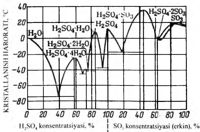
4.2-rasm. Sulfat kislotalarining kristallanish diagrammasi.
