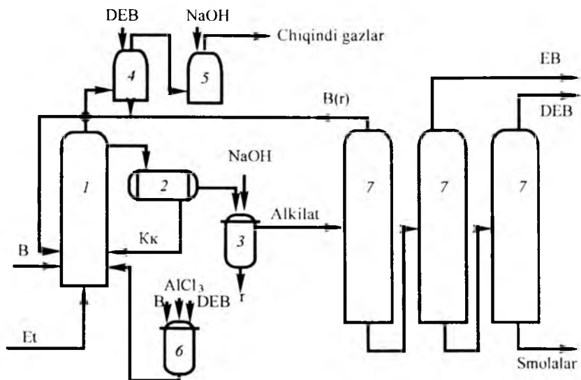
3.9-rasm. Benzolni etilen bilan alkillash jarayonining sxemasi:
