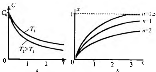
2.52-rasm. C(\tau) ning T_1 va T_2 > T_1 (a) va x(\tau) (b) temperaturalarda turli n tartibli reaksiyalarda va ideal aralashuv reaktoridagi bog'liqligi.
