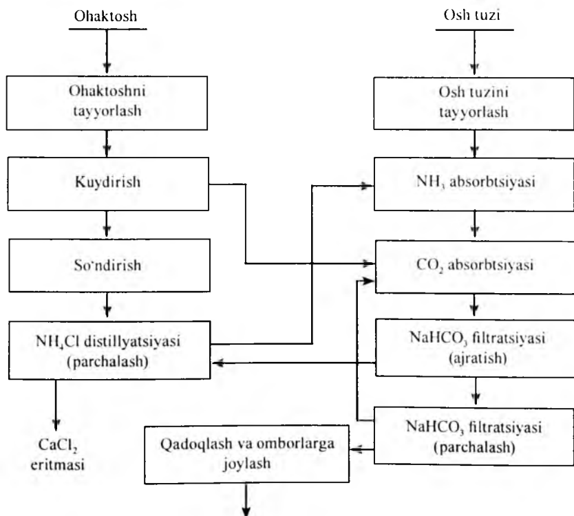
5.4-rasm. Soda ishlab chiqarish funktsional sxemasi
