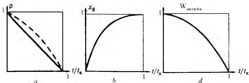
2.23-rasm. Vaqt t ning radiussiz zarracha \rho (a), qattiq reagent x_B (b) va zarracha W_{\text{zarracha}} (d) aylanish tezligining geterogen «siqiluvchi sfera» jarayoni uchun o'zgarishi. t_k – to'la aylanish vaqti. Punktir chiziq – \rho ning zarracha o'lchamining o'zgarishini massa almashinuv koeffitsiyenti \beta ta'siridagi o'zgarishi.
