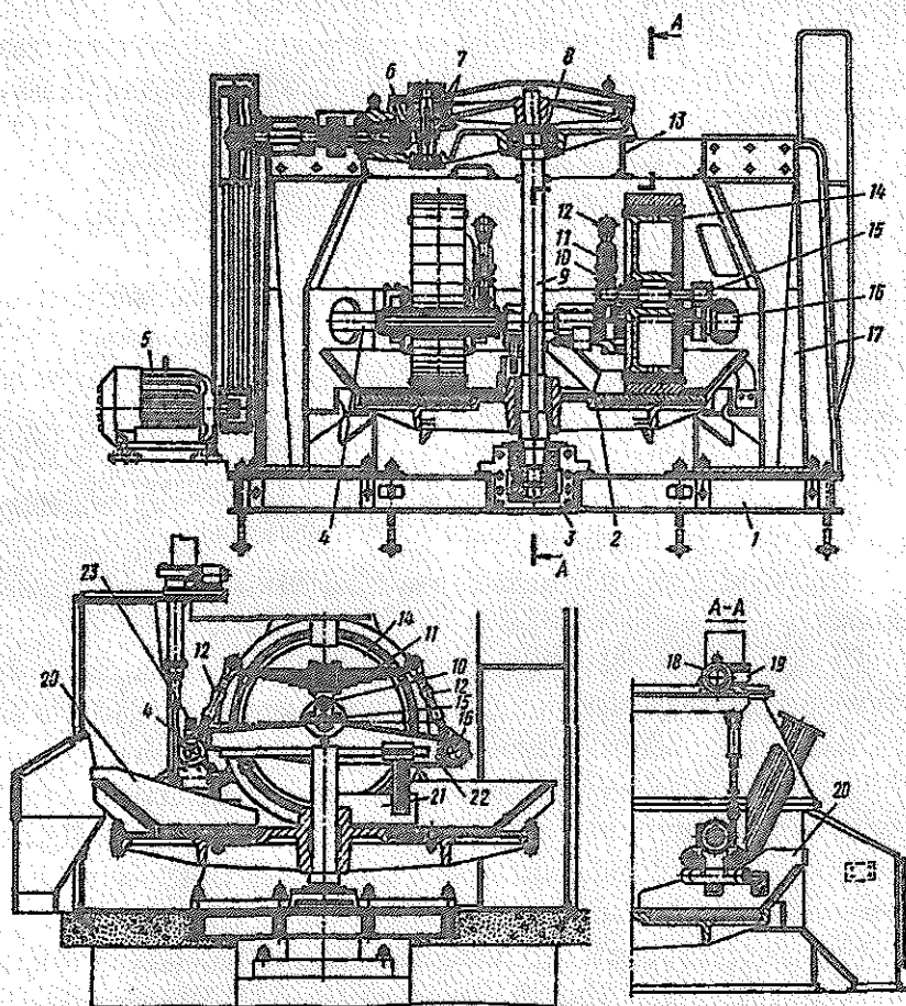
10-rasm. Prujinaning bosimi bilan sozlanadigan aralashtirgich begunlar:
