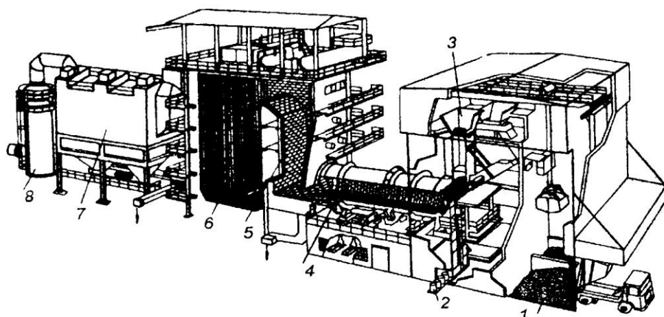
13- rasm. Zaharli sanoat chiqindilarini termik zararsizlantirish uchun agregat (MAN firmasi, Germaniya)
