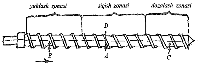
4-rasm. Chervyakning zonalarga bo'linishi.
