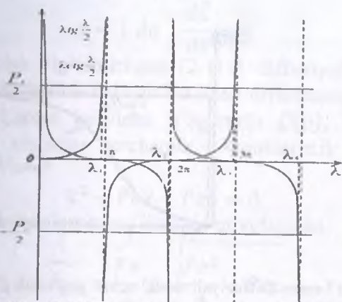
2.15-rasm. (2.109), (2.110) transcendent tenglamalar ildizlarining grafik talqini
