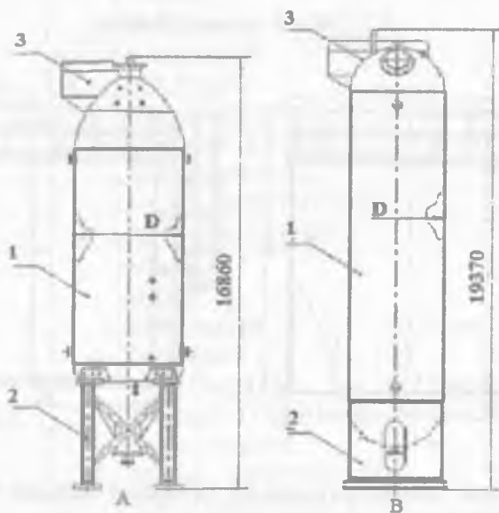
3.1-rasm. Akkumullovchi bak
