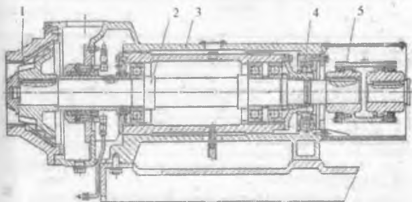
2.19-rasm. MII-00 rusumli pulsatsiyalovchi tegirmon: 1 – stator; 2 – rotor; 3 – stanina; 4 – tirqishni o'rnatish mexanizmi; 5 – tishli mufta.
