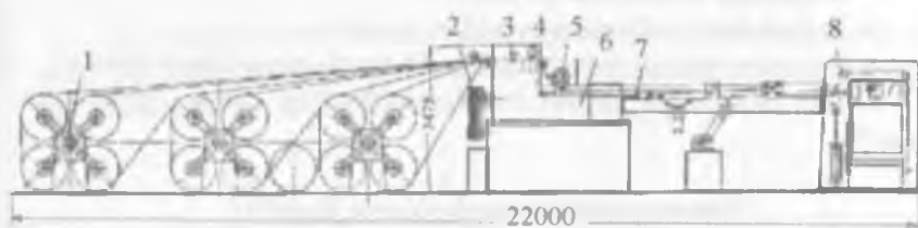
10.15-rasm. C1-13 rusumli polotnnoni ko'ndalangiga qirqish dastgohi:
