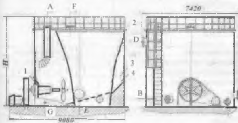
3.4-rasm. 204-135 rusumli havza.
