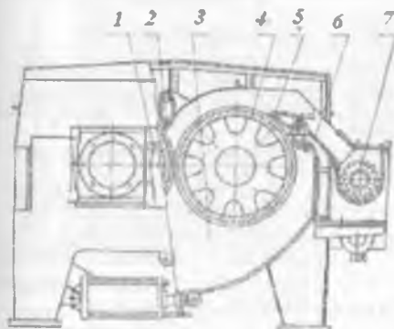
5.3-rasm. C2B-07-35 rusumli ikki barabanli quyultirgich:
