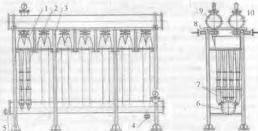
6.8-rasm. YBK-40-01, YBK-90-01, YBK-180-01, YBK-300-01 rusumli uyurmali tozalagich ko'rinishi:
