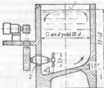
3.8-rasm. Vertikal mashina havzasi:
