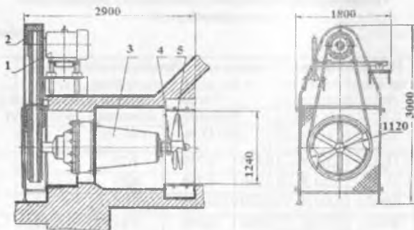
3.9-rasm. QY-10-02 rusumli sirkulatsiyalovchi qurilma (b): 1 – el. dvigatel; 2 – to'siq; 3 – korpus; 4 – val; 5 – vint.
