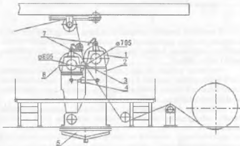
10.8-rasm. Yelimlash pressining sxemasi:
