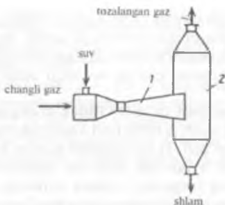
5.13-rasm. Venturi skrubberi: 1 – purkagich trubasi; 2 – siklon-changushlagich.
