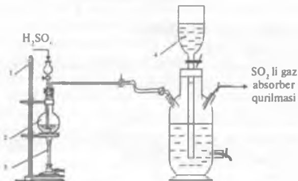
1-rasm. \text{SO}_2 gazini olish laboratoriya qurilmasi:
