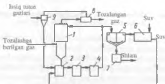
9.5- rasm. Kul suspenziyasi yordamida \text{SO}_2 gazini tozalash texnologik sxemasi:
