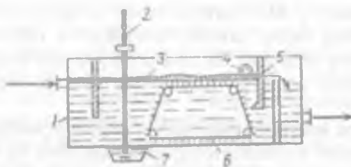
17.7-rasm. Neft ushlagich:
