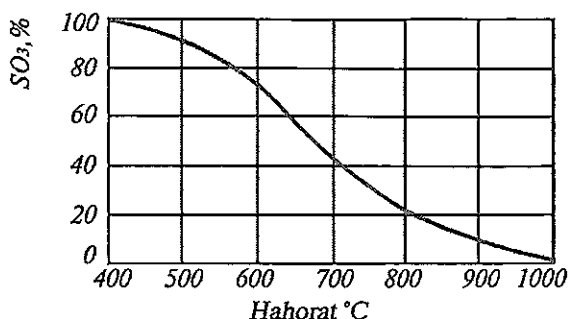
58- rasm. Tarkibida 7% \text{SO}_2 va 11 % \text{O}_2 saqllovchi \text{SO}_2 gazining 0,1 MPa bosimda oksidlanishining muvozanat darajasining haroratga bog'liqligi.
