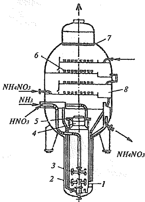
70-rasm. Neytrallanish issiqligidan foydalanish (NIF) reaktori.
