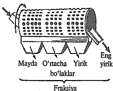
3- rasm. Baraban g'alvir.
