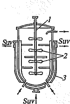
31- rasm. Parrakli aralashtirgichi bo'lgan reaktor.
