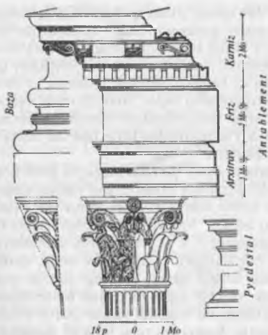
14-rasm. Korinf ordeni.
