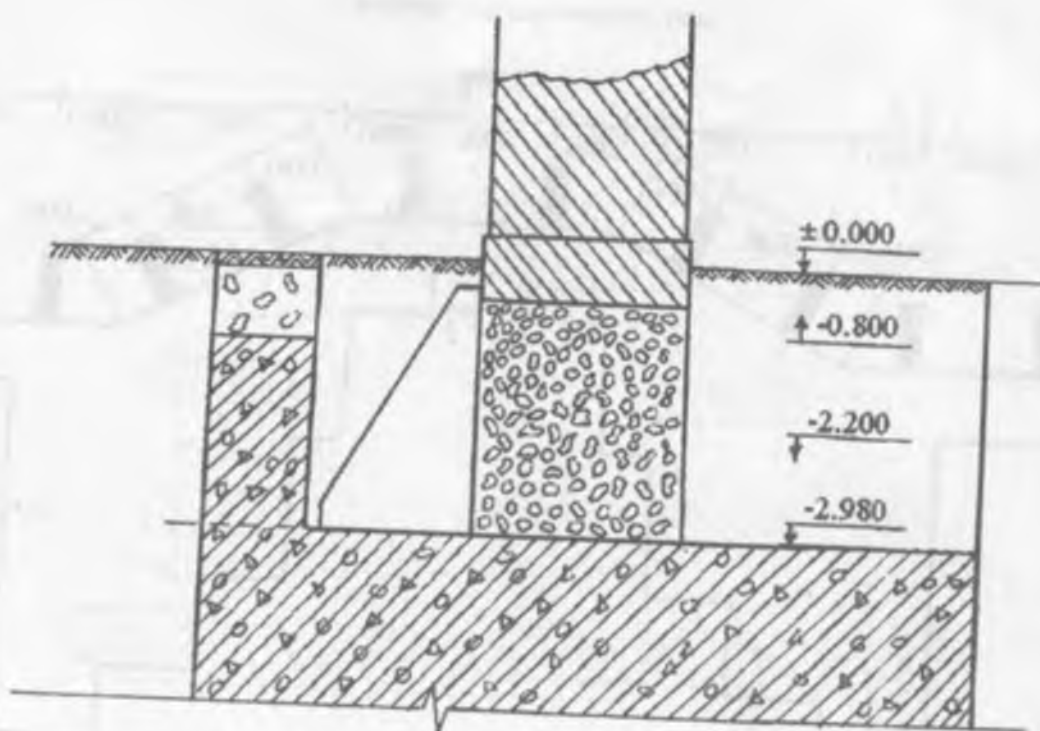
4-rasm. Poydevor qirgimi.
