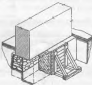
3.7.6-rasm. Devor tagiga temirbeton o'rnatish.
