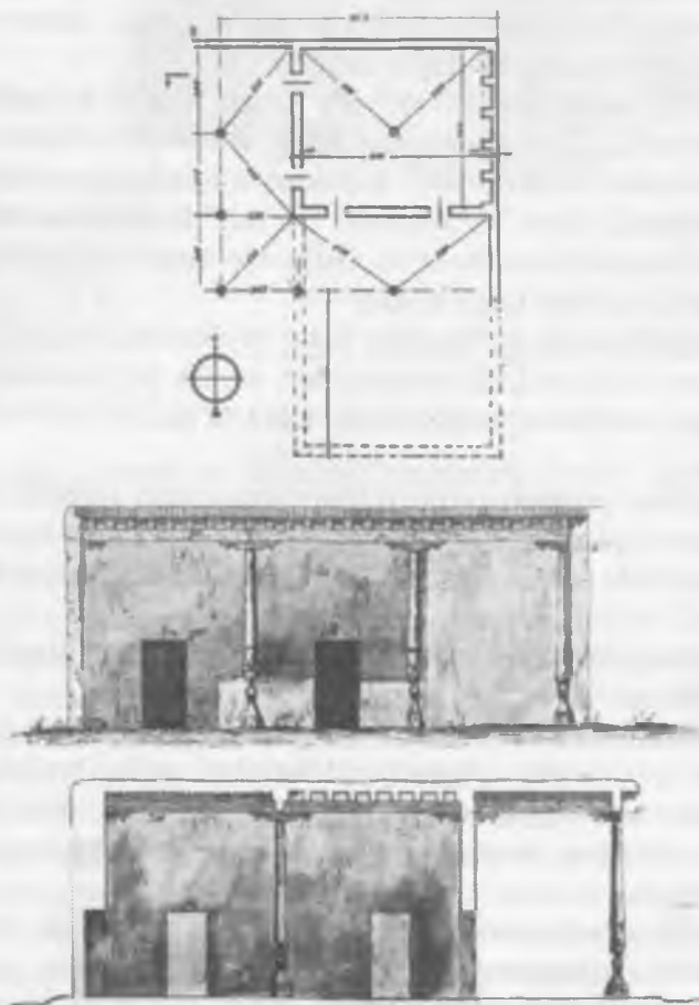
6.4.1-rasm. Guzar masjidi, tarh, tarz, qirqim chizmalari.
